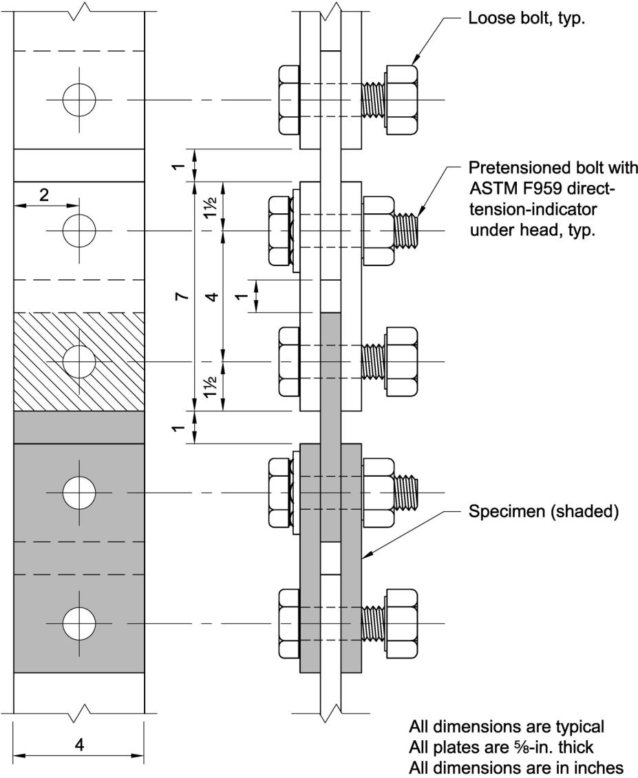
Figure A-2. Creep test specimen assembly.
